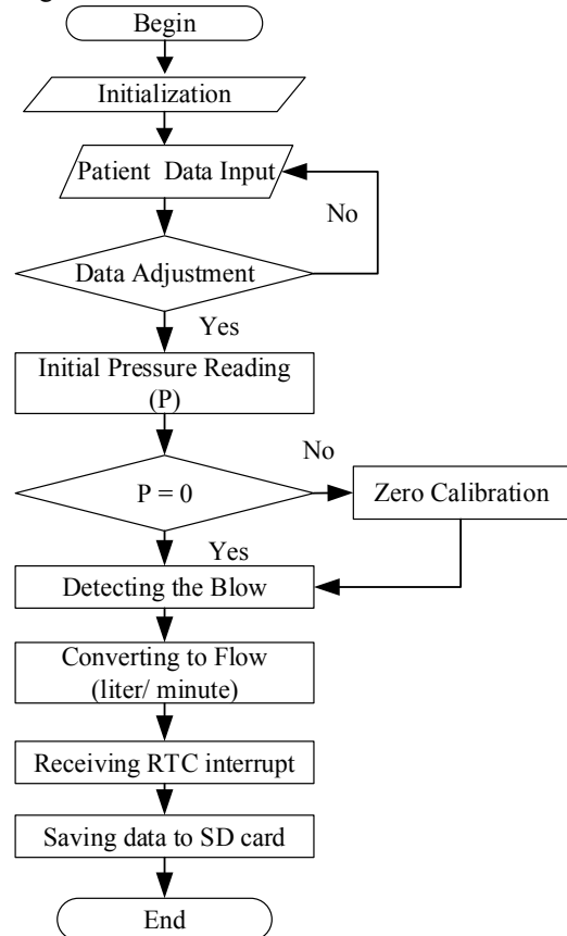
FIGURE 2. The Flowchart of The Arduino Program
