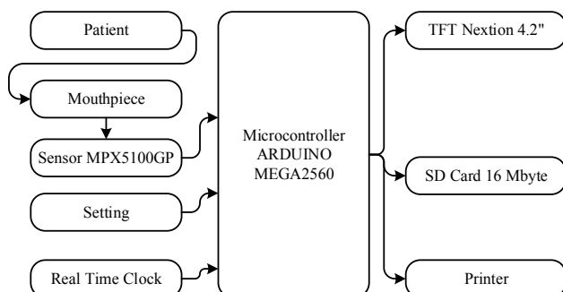
FIGURE 1. The Block Diagram of Peak Flow Meter
