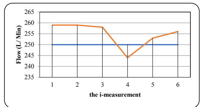
FIGURE 4. Result Of Measurement Of Flow Value At A Pressure 1,4 Kg/Cm 2 . (The orange line indicates the design and the blue line indicates the standard unit)
