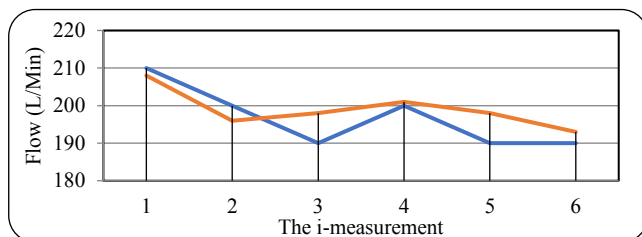
FIGURE 3. Result of Measurement Of Flow Value At A Pressure 0,7 Kg/Cm 2 . (The orange line indicates the design and the blue line indicates the standard unit)
